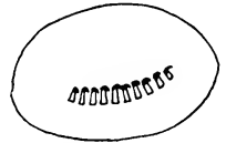
Fig. 427. Crochets in single band.
